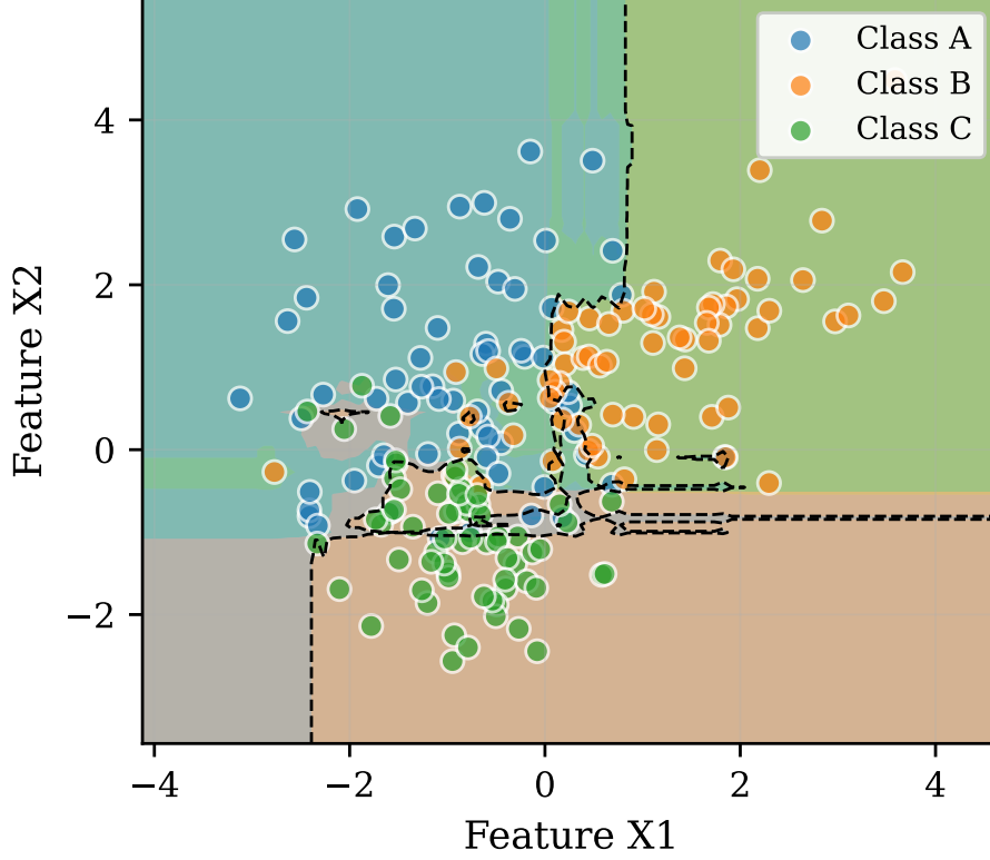
Figure 2: Decision boundaries in a multi-class classification problem.
