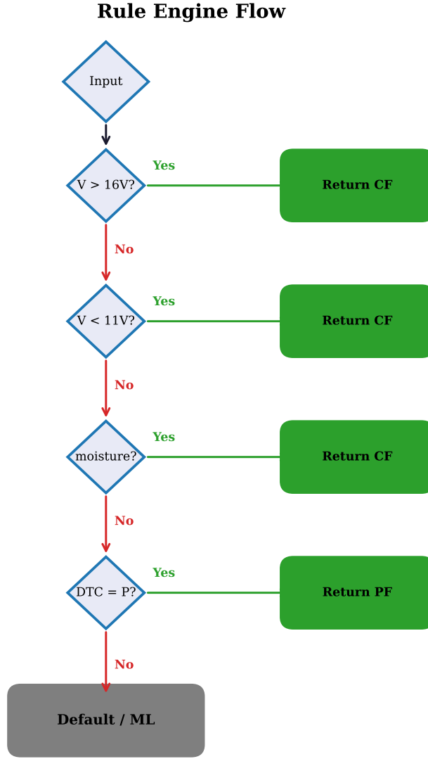
Figure 16: Deterministic rule engine: rules evaluated in priority order; first match fires.
